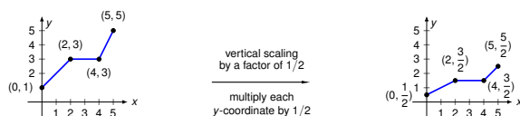
Figure 46: Graphs of y = f(x) and y = \frac{1}{2}f(x)
