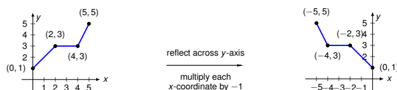
Figure 35: Graphs of y = f(x) (left) and y = f(-x) (right).
