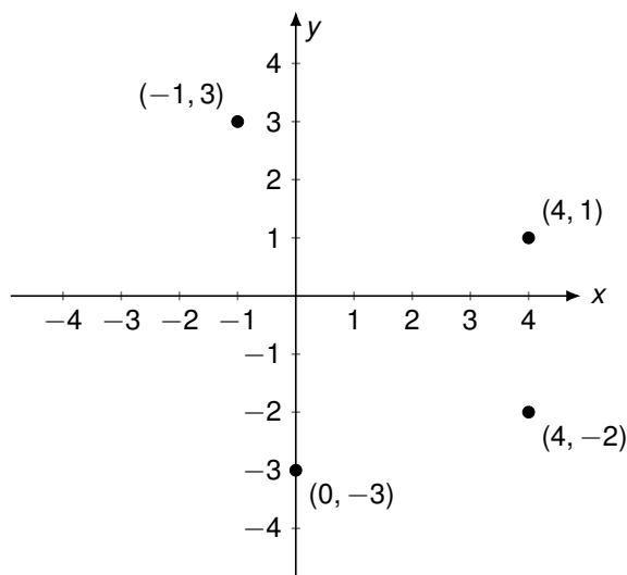
Figure 54: The graph of R
