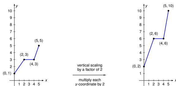
Figure 45: Graphs of y = f(x) and y = 2f(x)
