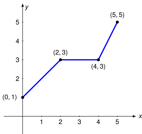
Figure 44: y = f(x)
