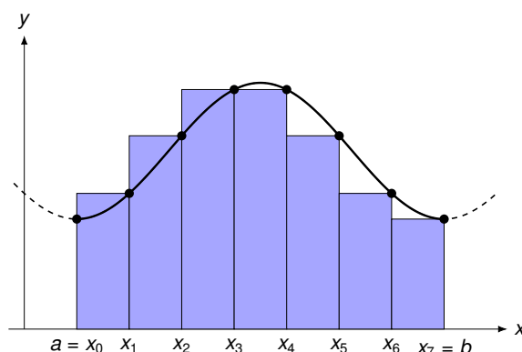
Figure 59: Visualizing RS_7 , a 'right endpoint sum.'
