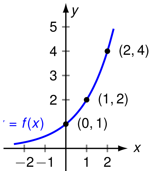
Figure 36: Graph of y = f(x)
