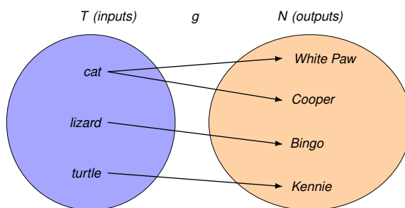
Figure 52: Mapping diagram for g
