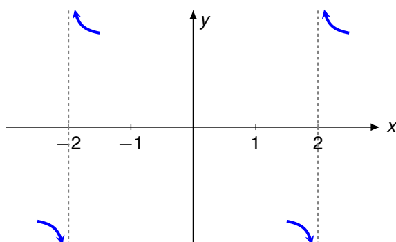
Figure 10: Behavior near x = \pm 2
