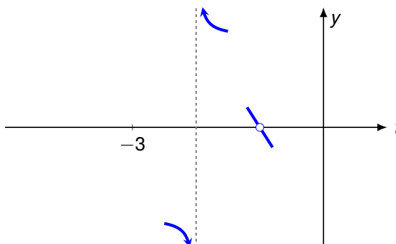
Figure 18: Behavior near x = -2 and x = -1
