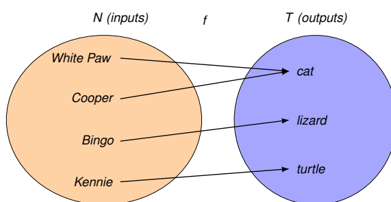
Figure 51: Mapping diagram for f
