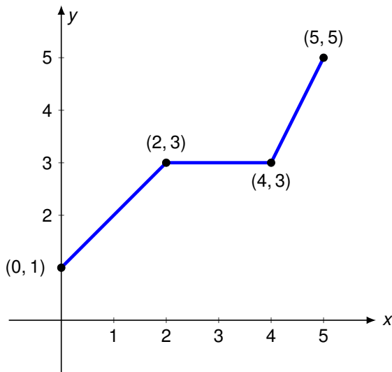
Figure 25: y = f(x)
