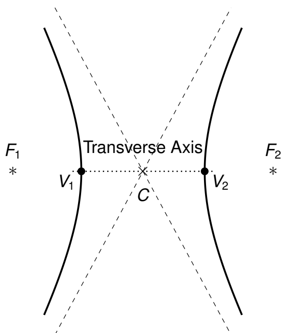
Figure 57: A hyperbola with center C ; foci F_1 , F_2 ; and vertices V_1 , V_2 and asymptotes (dashed)
