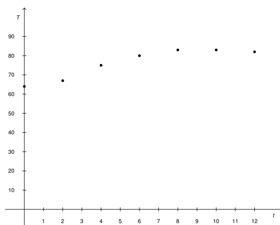
Figure 4: The graph of T = f(t)
