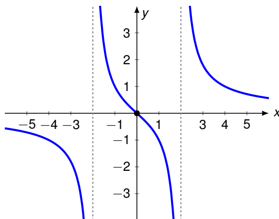
Figure 13: Graph of y = f(x)
