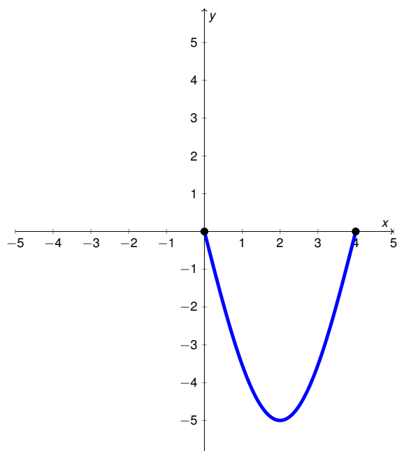
Partial graph of y = f(x)
