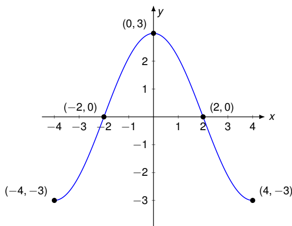
Figure 49: Graph of y = f(x)
