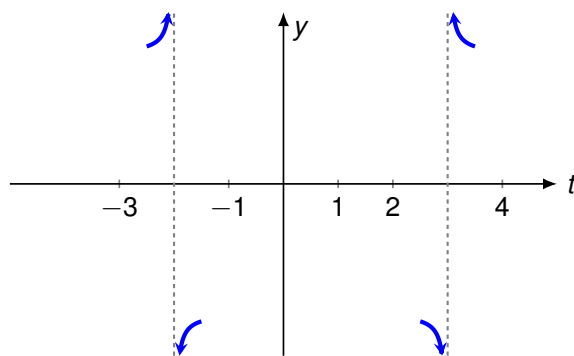
Figure 14: Behavior near t = -2 and t = 3
