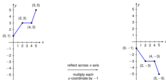
Figure 34: Graphs of y = f(x) (left) and y = -f(x) (right).
