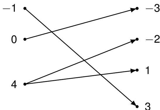
Figure 53: Mapping diagram for R
