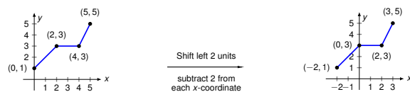
Figure 27: Graphs of y = f(x) (left) and y = g(x) = f(x + 2) (right).
