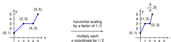
Figure 47: Graphs of y = f(x) and y = f(2x)
