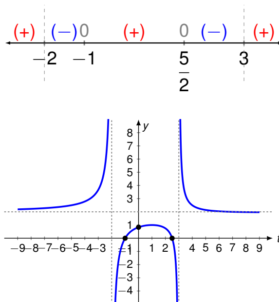
Figure 17: Graph of y = g(t)
