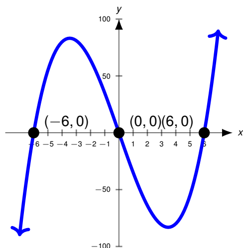
The graph of y = f(x) .
