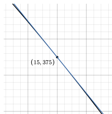
Zooming in closer to (15, 375) .
