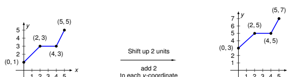
Figure 26: Graphs of y = f(x) (left) and y = g(x) = f(x) + 2 (right).
