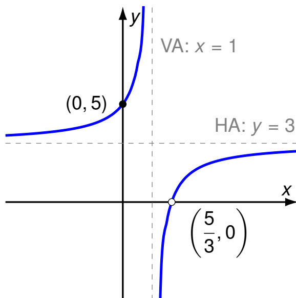
Figure 23: Graph of y = F(x)
