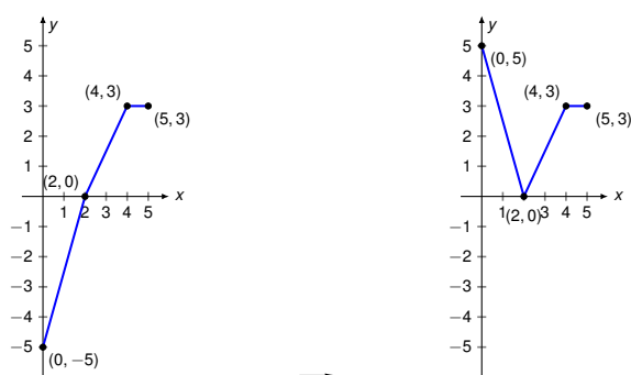
Figure 50: Graphs of y = f(x) and y = g(x)
