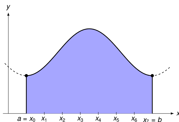
Figure 58: Area under the graph of y = f(x) .
