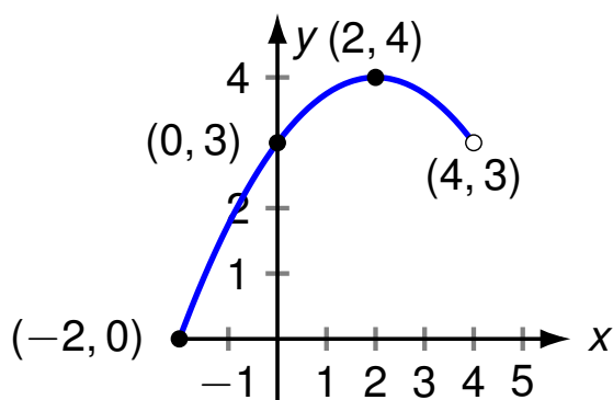
Figure 28: Graph of y = f(x) .
