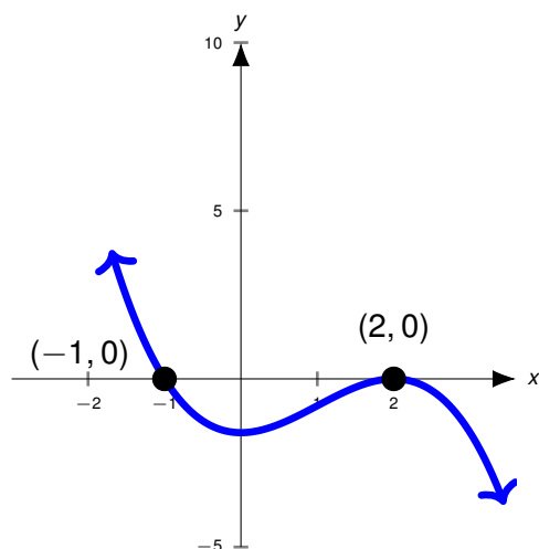
The graph of y = p(z) .
